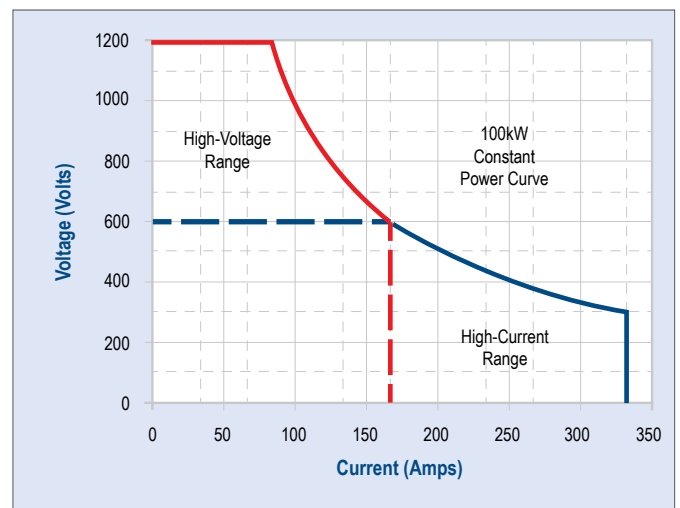
Figure 1 - Wide Constant Power Operating Envelope
